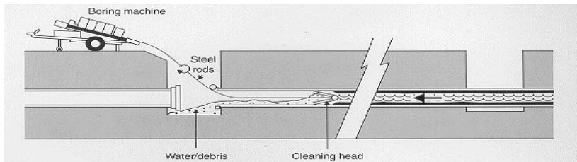
Figure CP1.1 Power Boring - diameter range 75mm to 250mm: to remove debris and encrustation from the pipe
