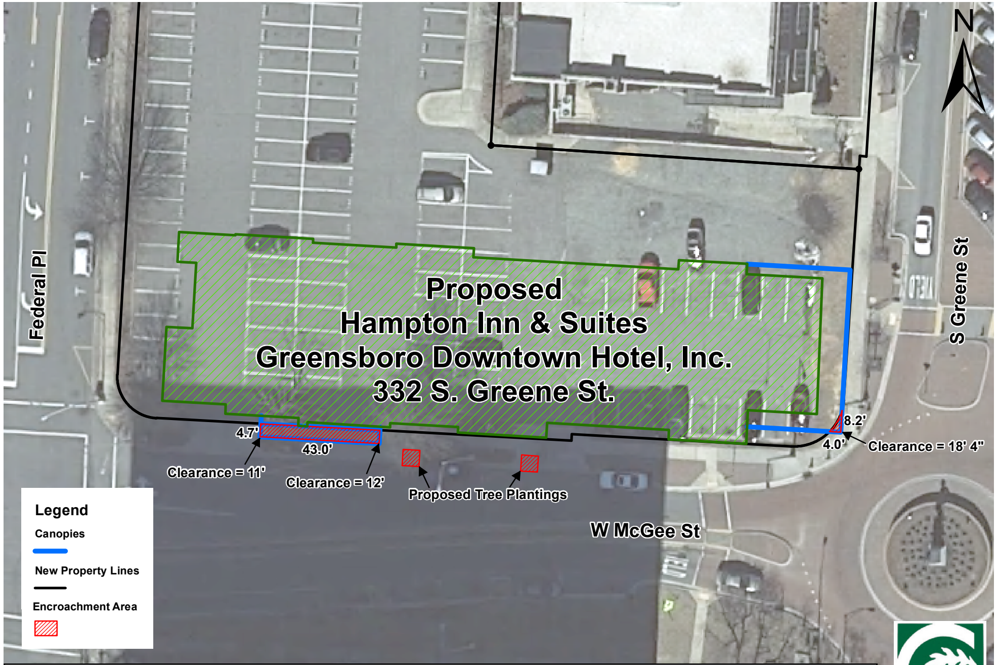
SITE PLAN WITH PROPOSED ENCROACHMENT IN CITY RIGHT-OF-WAY For Hampton Inn & Suites - 332 S. Greene St. - Use of City Right of Way for Proposed Canopies & Trees
